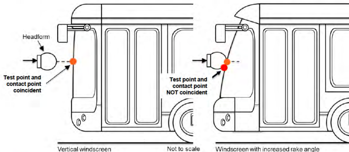
Figure 36_7: Test point and head-form contact point not coincident for impacts against surface not normal to direction of propulsion
